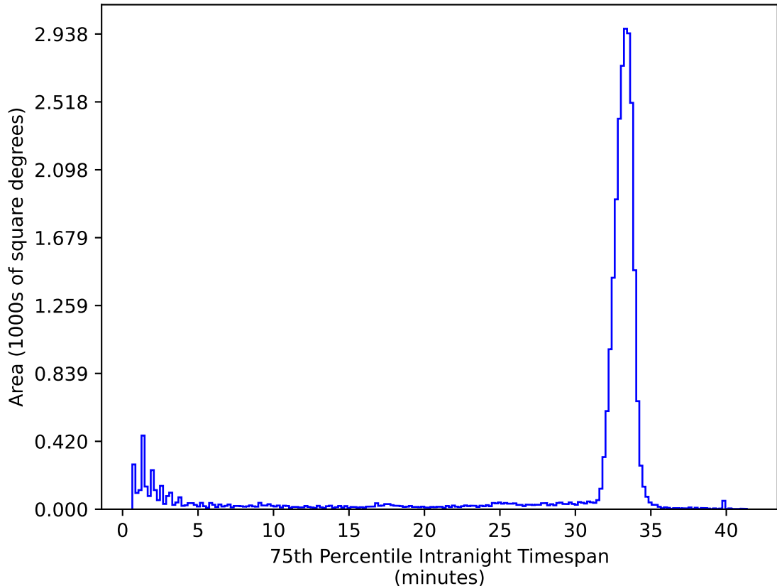
ddf_acor_sf10_lsf20_lsr10_v3.4_10yrs All sky ug bands: 75th Percentile Intranight Timespan
