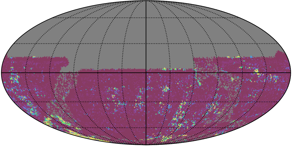
ddf_acor_sf10_lsf20_lsr10_v3.4_10yrs All sky u band: 75th Percentile Intranight Timespan
