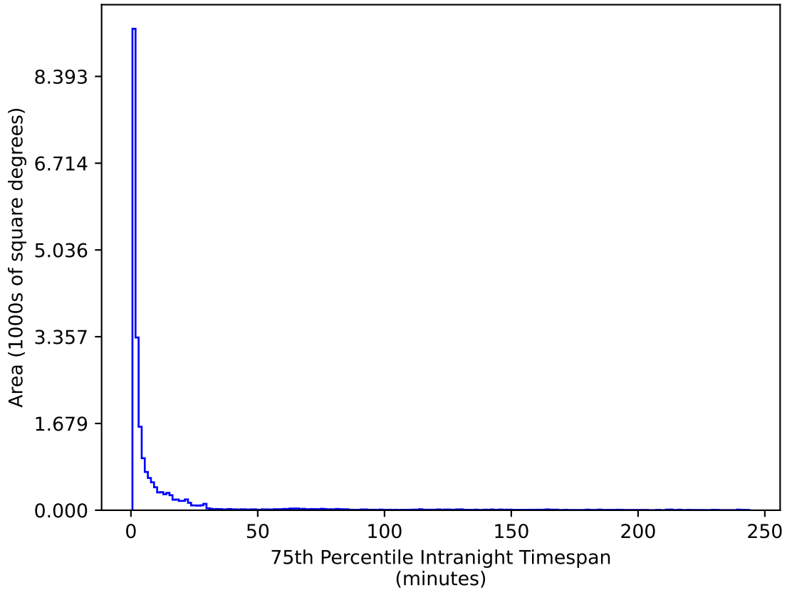
ddf_acor_sf10_lsf20_lsr10_v3.4_10yrs All sky u band: 75th Percentile Intranight Timespan
