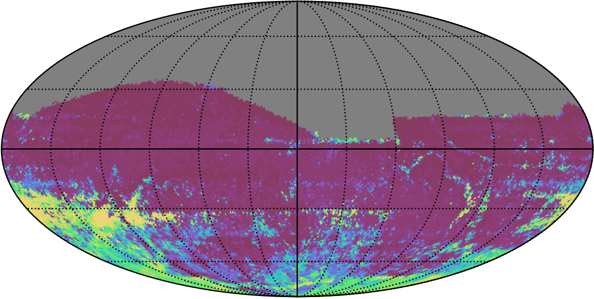
ddf_acor_sf10_lsf20_lsr10_v3.4_10yrs All sky r band: 75th Percentile Intranight Timespan
