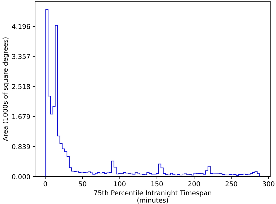
ddf_acor_sf10_lsf20_lsr10_v3.4_10yrs All sky r band: 75th Percentile Intranight Timespan
