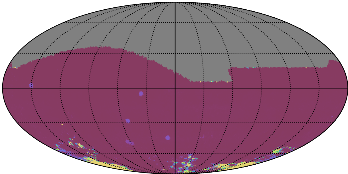
ddf_acor_sf10_lsf20_lsr10_v3.4_10yrs All sky iz bands: 75th Percentile Intranight Timespan
