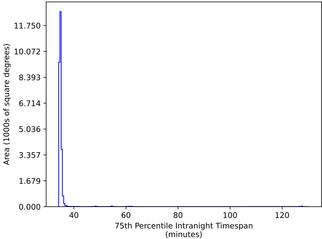
ddf_acor_sf10_lsf20_lsr10_v3.4_10yrs All sky iz bands: 75th Percentile Intranight Timespan
