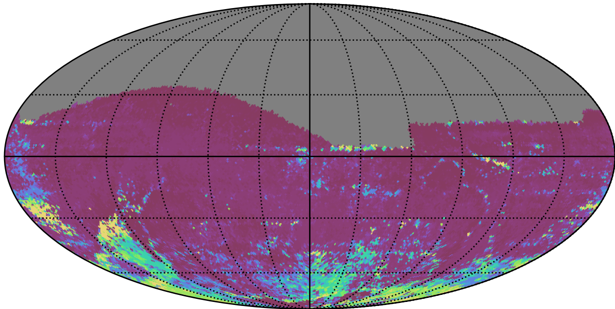
ddf_acor_sf10_lsf20_lsr10_v3.4_10yrs All sky i band: 75th Percentile Intranight Timespan
