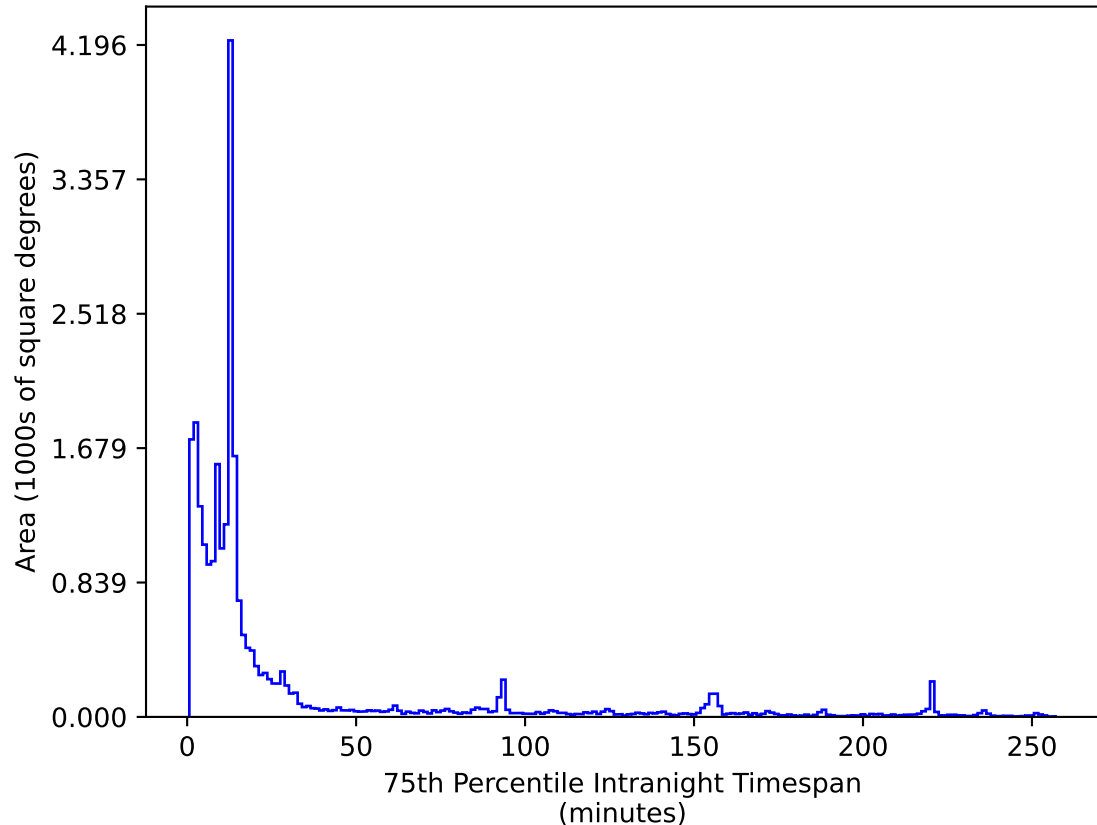
ddf_acor_sf10_lsf20_lsr10_v3.4_10yrs All sky i band: 75th Percentile Intranight Timespan
