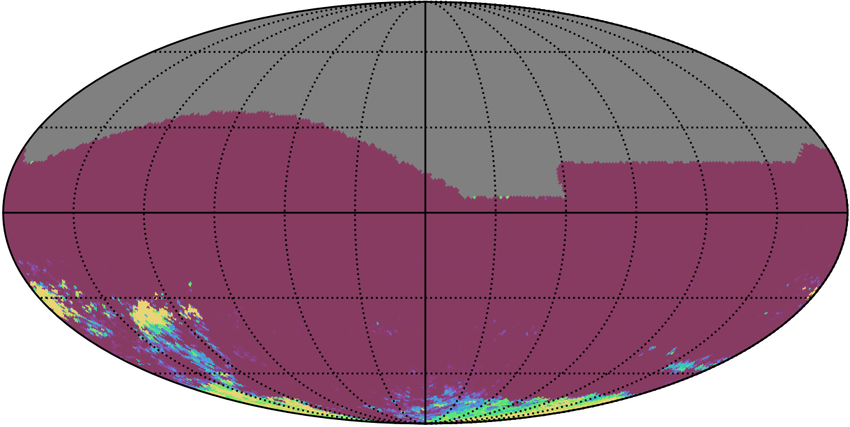
ddf_acor_sf10_lsf20_lsr10_v3.4_10yrs All sky gr bands: 75th Percentile Intranight Timespan
