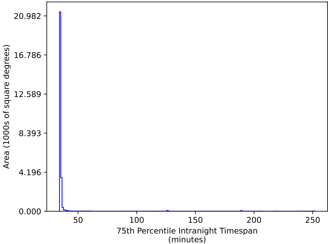
ddf_acor_sf10_lsf20_lsr10_v3.4_10yrs All sky gr bands: 75th Percentile Intranight Timespan
