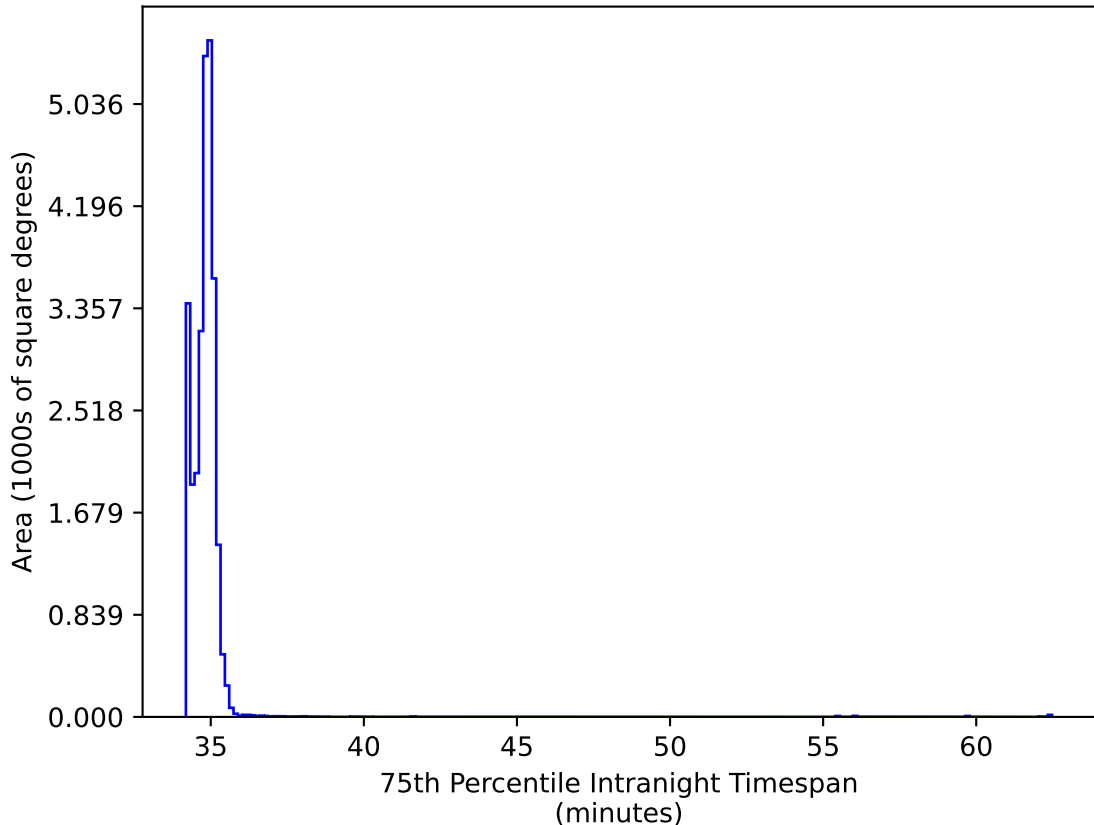
ddf_acor_sf10_lsf20_lsr10_v3.4_10yrs All sky all bands: 75th Percentile Intranight Timespan
