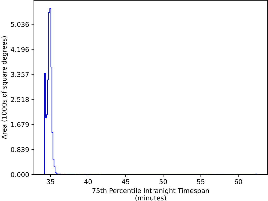
ddf_acor_sf10_lsf20_lsr10_v3.4_10yrs All sky: 75th Percentile Intranight Timespan
