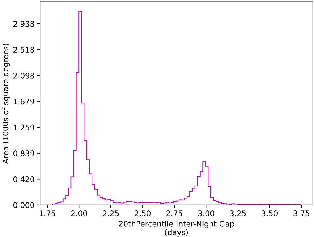
ddf_acor_sf10_lsf20_lsr10_v3.4_10yrs WFD z band: 20thPercentile Inter-Night Gap
