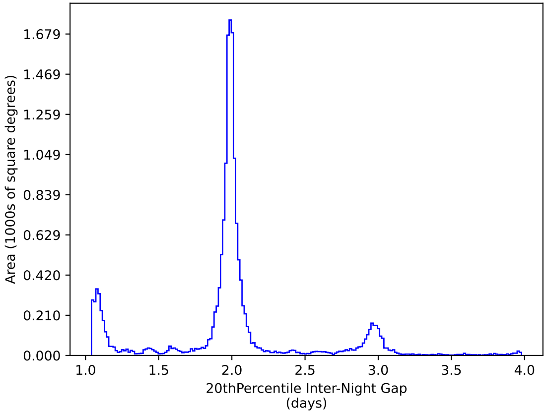
ddf_acor_sf10_lsf20_lsr10_v3.4_10yrs WFD y band: 20thPercentile Inter-Night Gap
