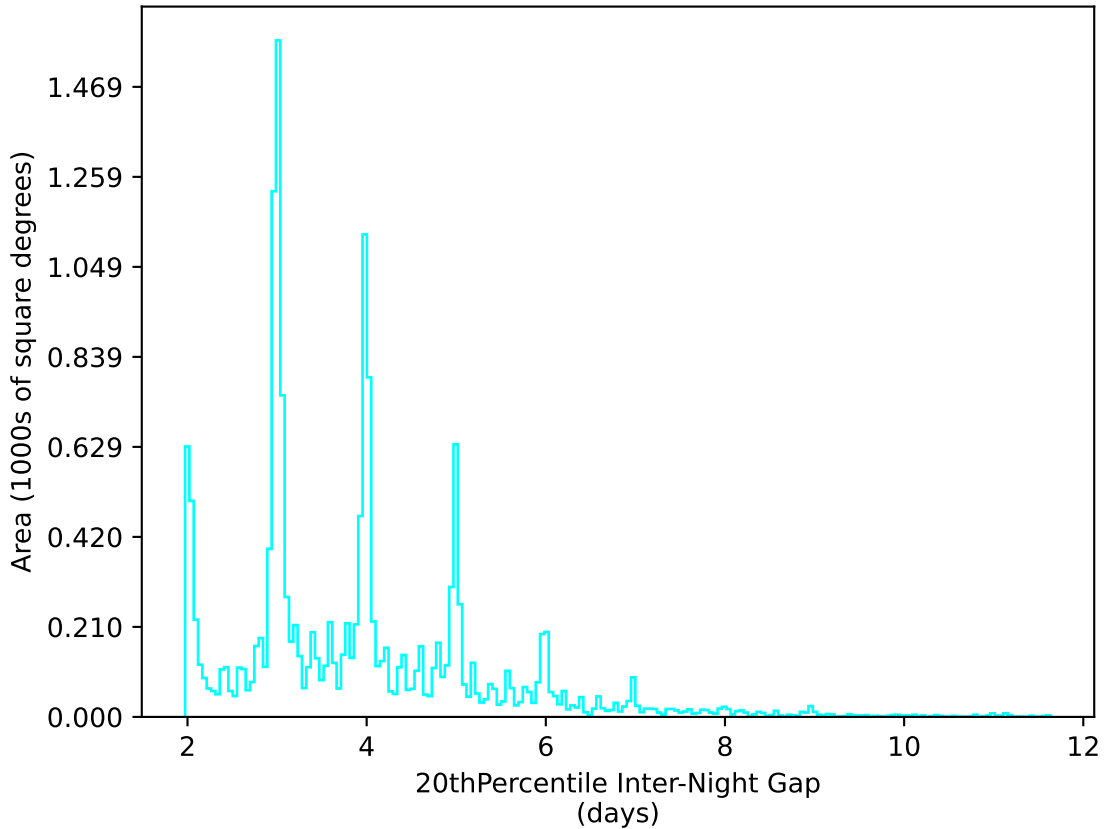
ddf_acor_sf10_lsf20_lsr10_v3.4_10yrs WFD u band: 20thPercentile Inter-Night Gap
