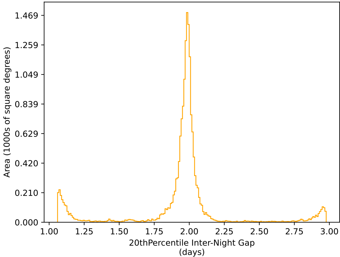
ddf_acor_sf10_lsf20_lsr10_v3.4_10yrs WFD r band: 20thPercentile Inter-Night Gap
