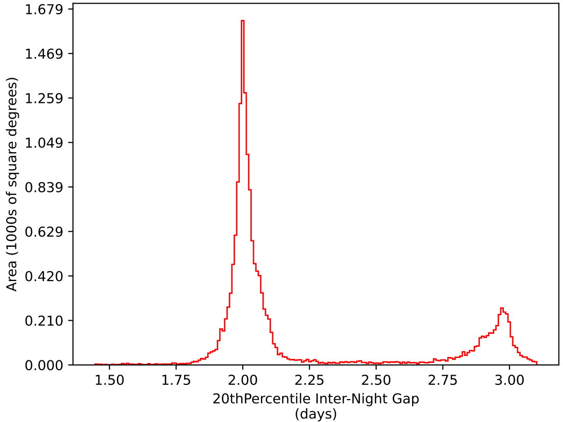
ddf_acor_sf10_lsf20_lsr10_v3.4_10yrs WFD i band: 20thPercentile Inter-Night Gap
