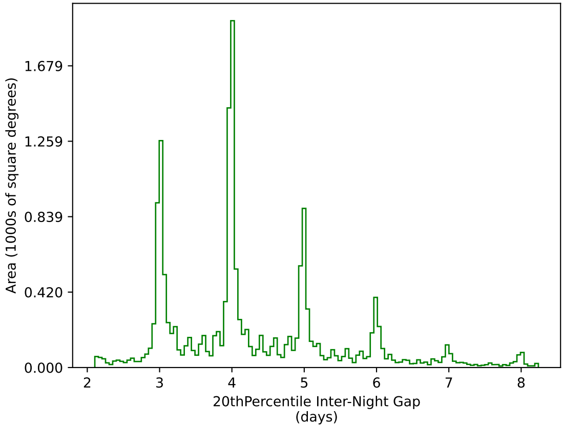
ddf_acor_sf10_lsf20_lsr10_v3.4_10yrs WFD g band: 20thPercentile Inter-Night Gap
