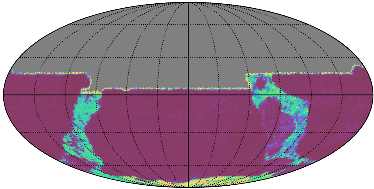
ddf_acor_sf10_lsf20_lsr10_v3.4_10yrs All sky y band: 20thPercentile Inter-Night Gap
