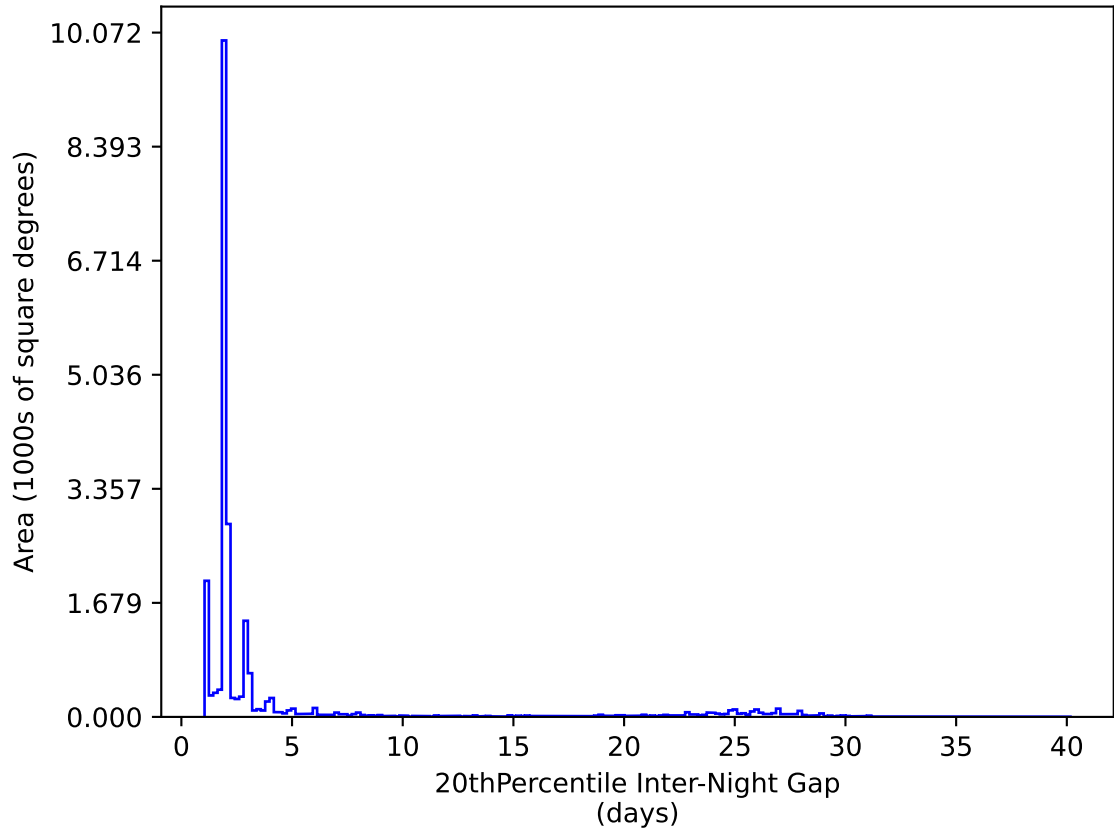
ddf_acor_sf10_lsf20_lsr10_v3.4_10yrs All sky y band: 20thPercentile Inter-Night Gap
