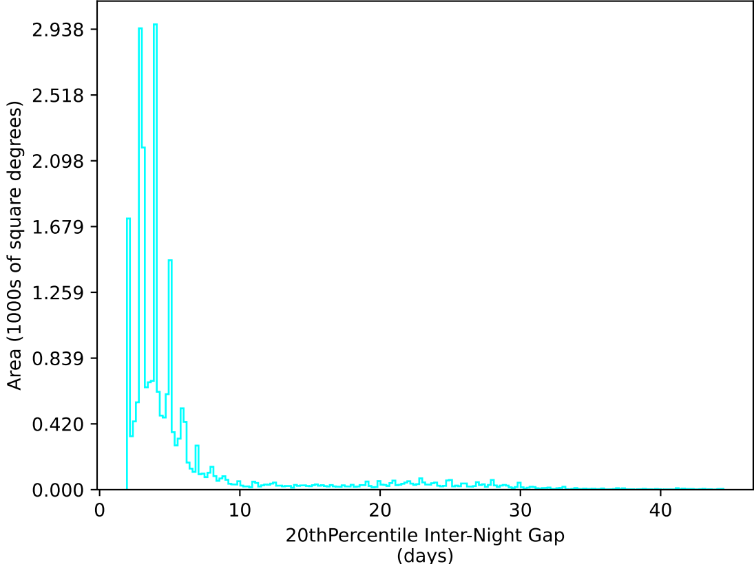
ddf_acor_sf10_lsf20_lsr10_v3.4_10yrs All sky u band: 20thPercentile Inter-Night Gap
