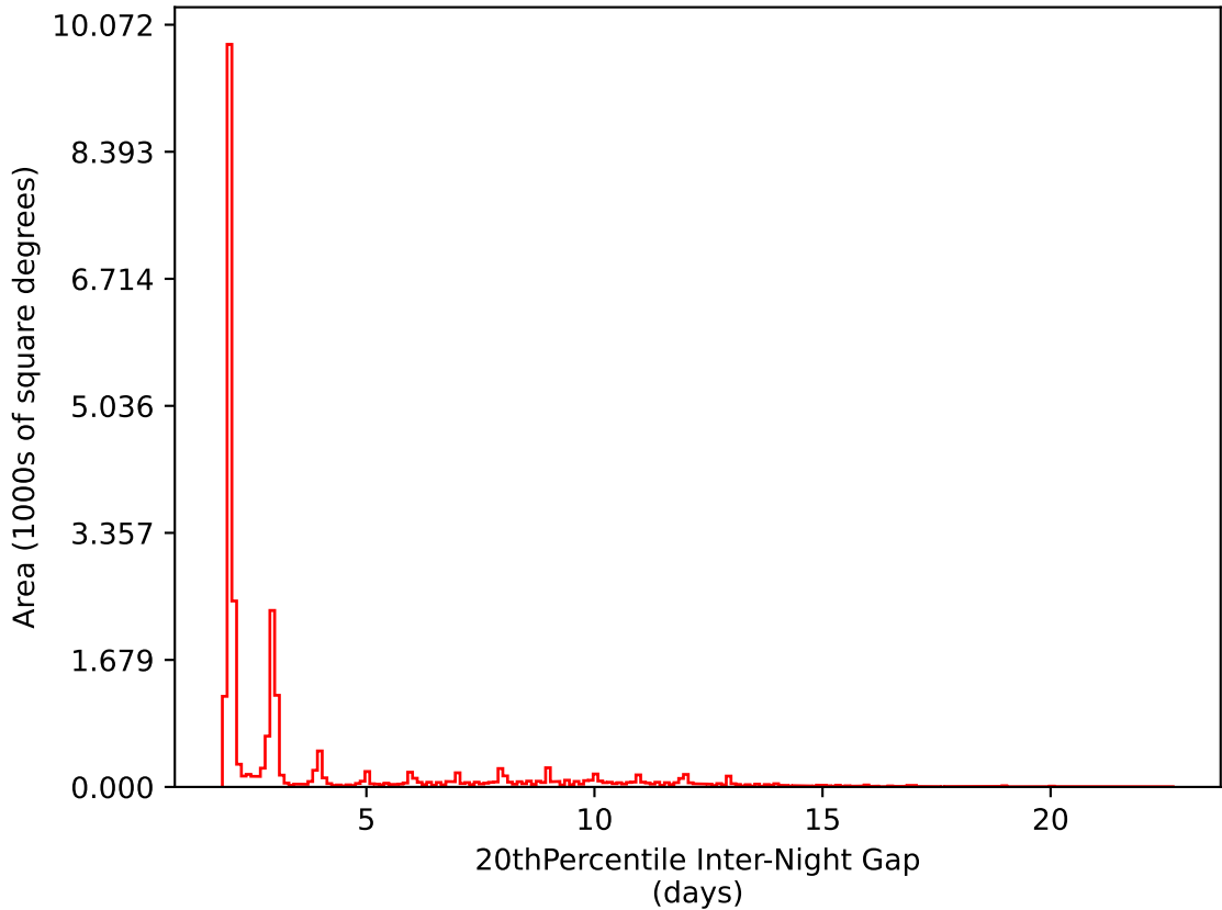
ddf_acor_sf10_ls20_lsr10_v3.4_10yrs All sky i band: 20thPercentile Inter-Night Gap
