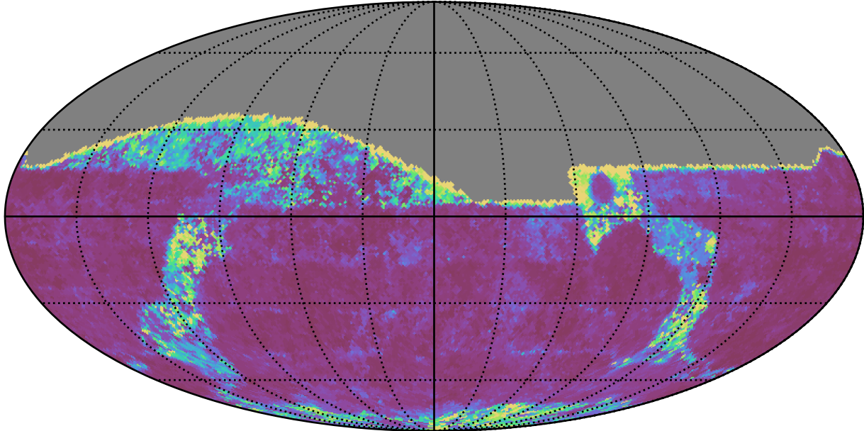
ddf_acor_sf10_lsf20_lsr10_v3.4_10yrs All sky g band: 20thPercentile Inter-Night Gap
