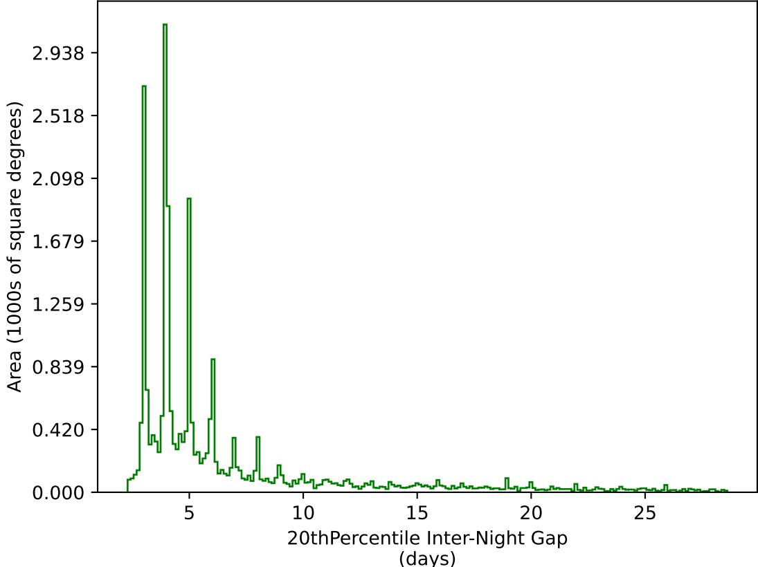
ddf_acor_sf10_lsf20_lsr10_v3.4_10yrs All sky g band: 20thPercentile Inter-Night Gap
