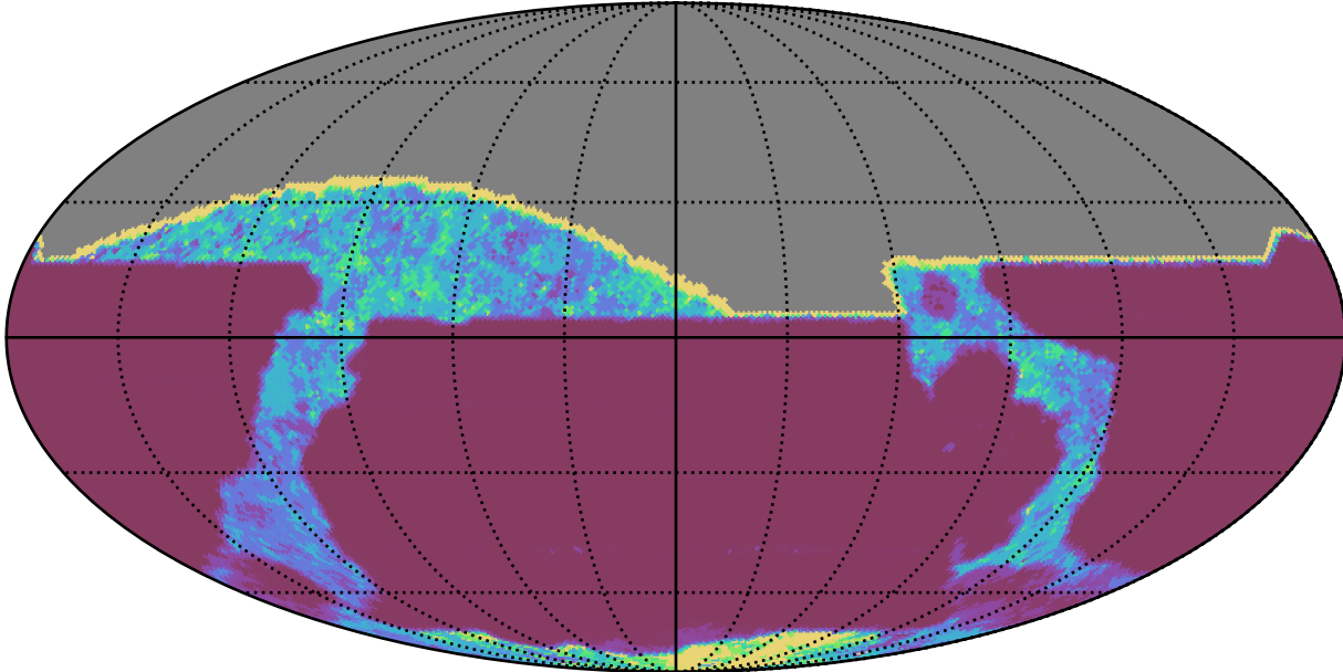
ddf_acor_sf10_lsf20_lsr10_v3.4_10yrs All sky all bands: 20thPercentile Inter-Night Gap
