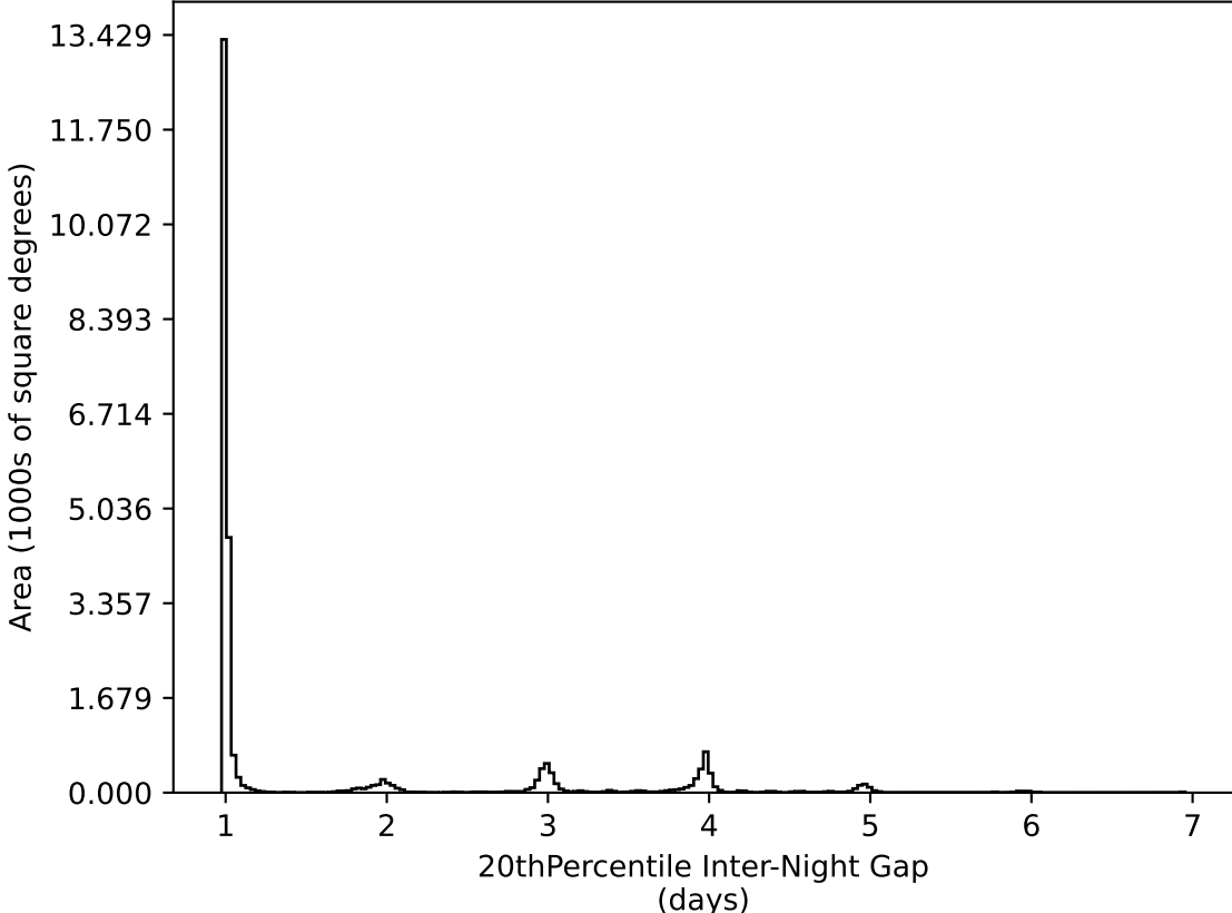
ddf_acor_sf10_lsf20_lsr10_v3.4_10yrs All sky all bands: 20thPercentile Inter-Night Gap
