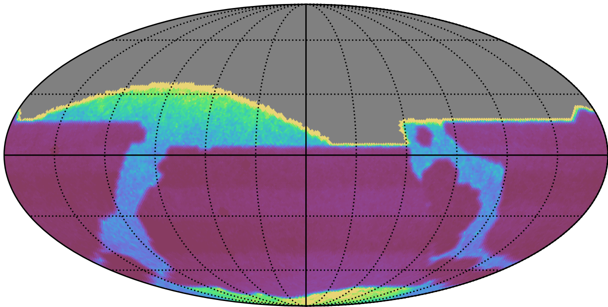
ddf_acor_sf10_lsf20_lsr10_v3.4_10yrs : properMotion
