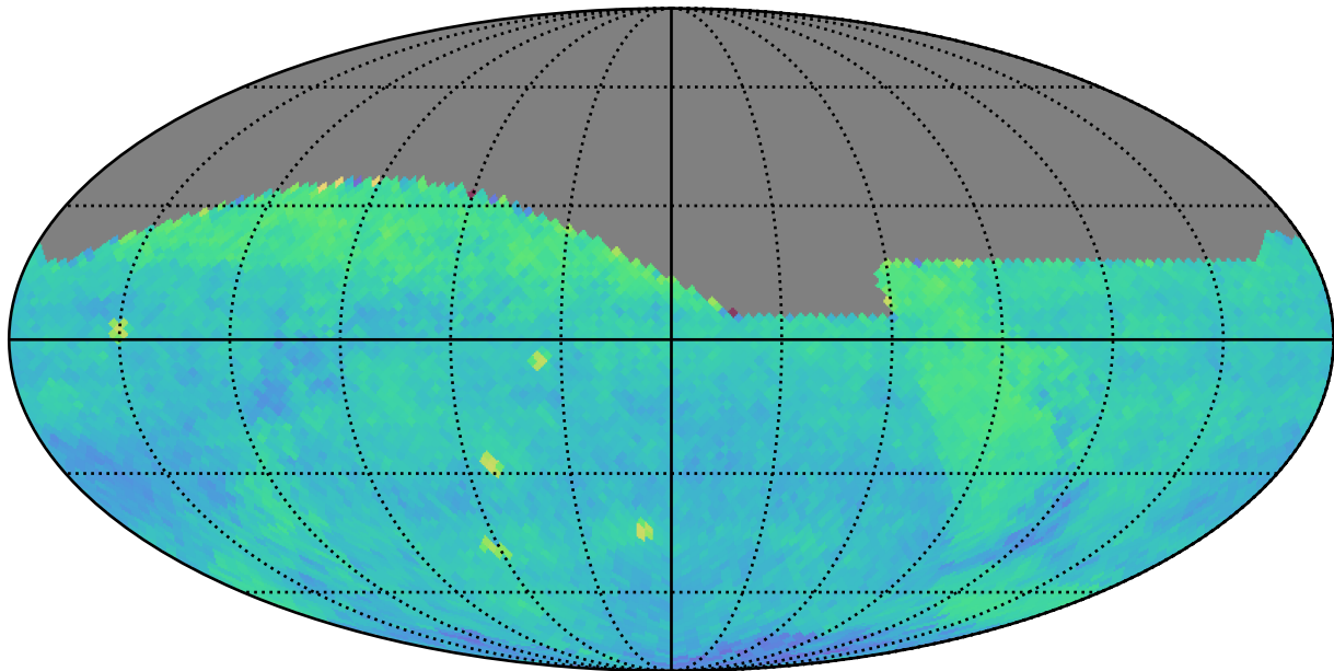
ddf_acor_sf10_lsf20_lsr10_v3.4_10yrs (g or r or i): PairFraction
