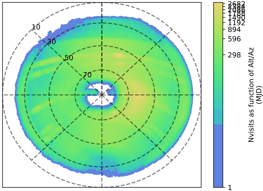
ddf_acor_sf10_lsf20_lsr10_v3.4_10yrs z: Nvisits as function of Alt/Az
