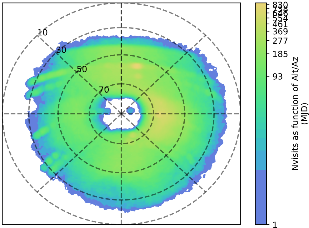
ddf_acor_sf10_lsf20_lsr10_v3.4_10yrs u: Nvisits as function of Alt/Az
