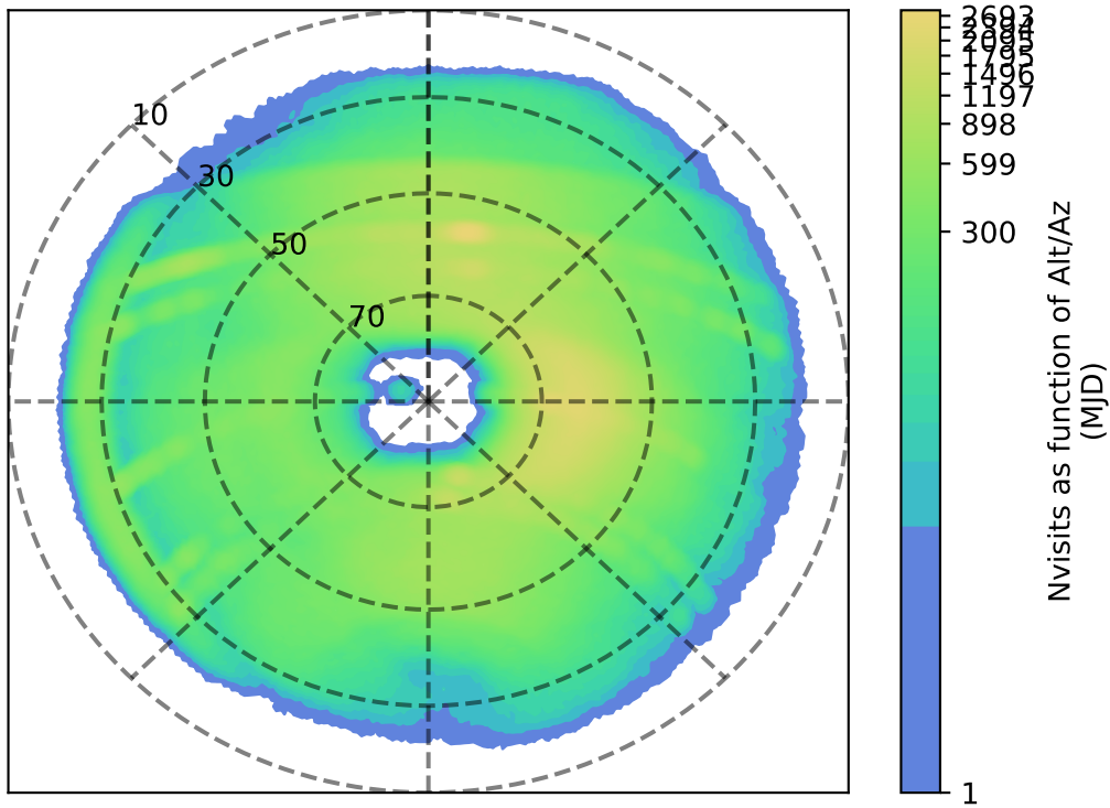
ddf_acor_sf10_ls20_lsr10_v3.4_10yrs r: Nvisits as function of Alt/Az
