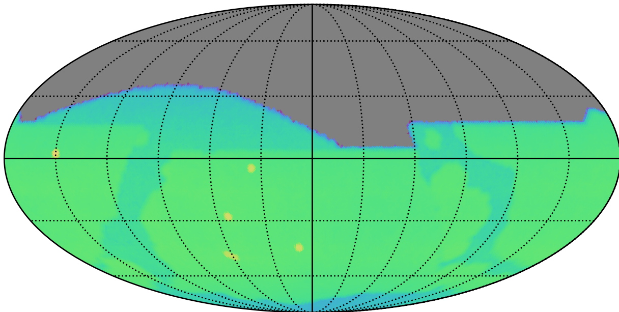
ddf_acor_sf10_lsf20_lsr10_v3.4_10yrs : CoaddM5
