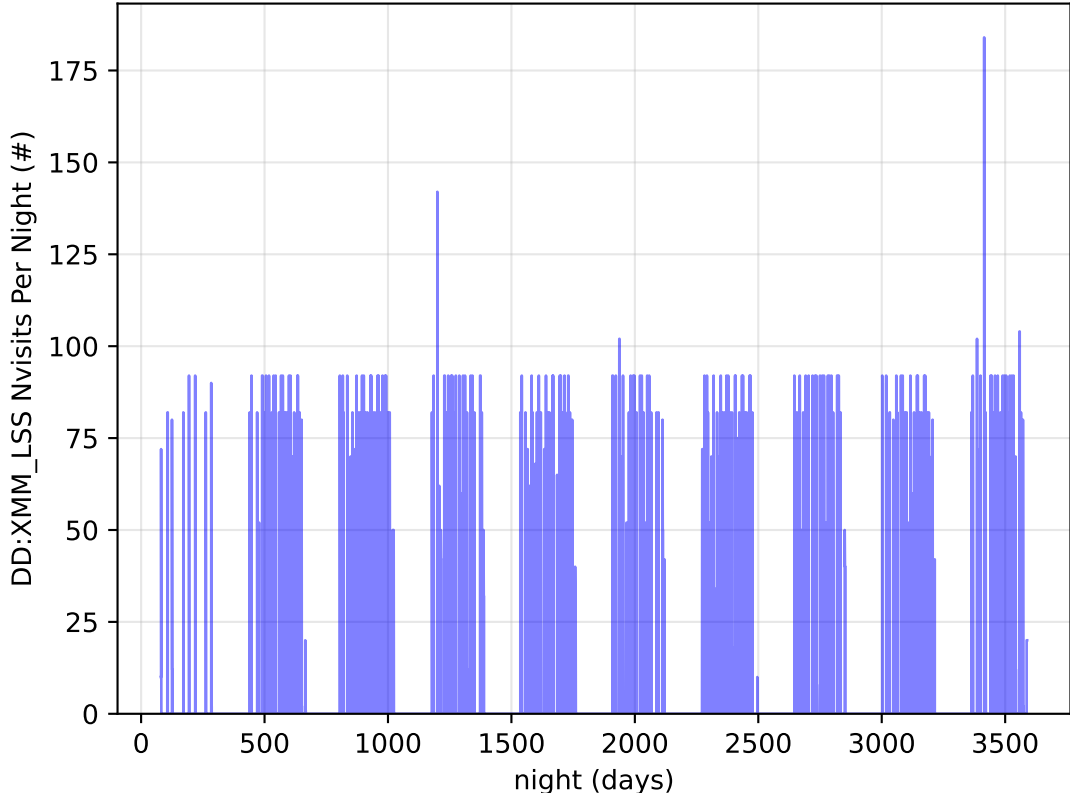
ddf_acor_sf10_lsf20_lsr10_v3.4_10yrs all bands: DD:XMM_LSS Nvisits Per Night
