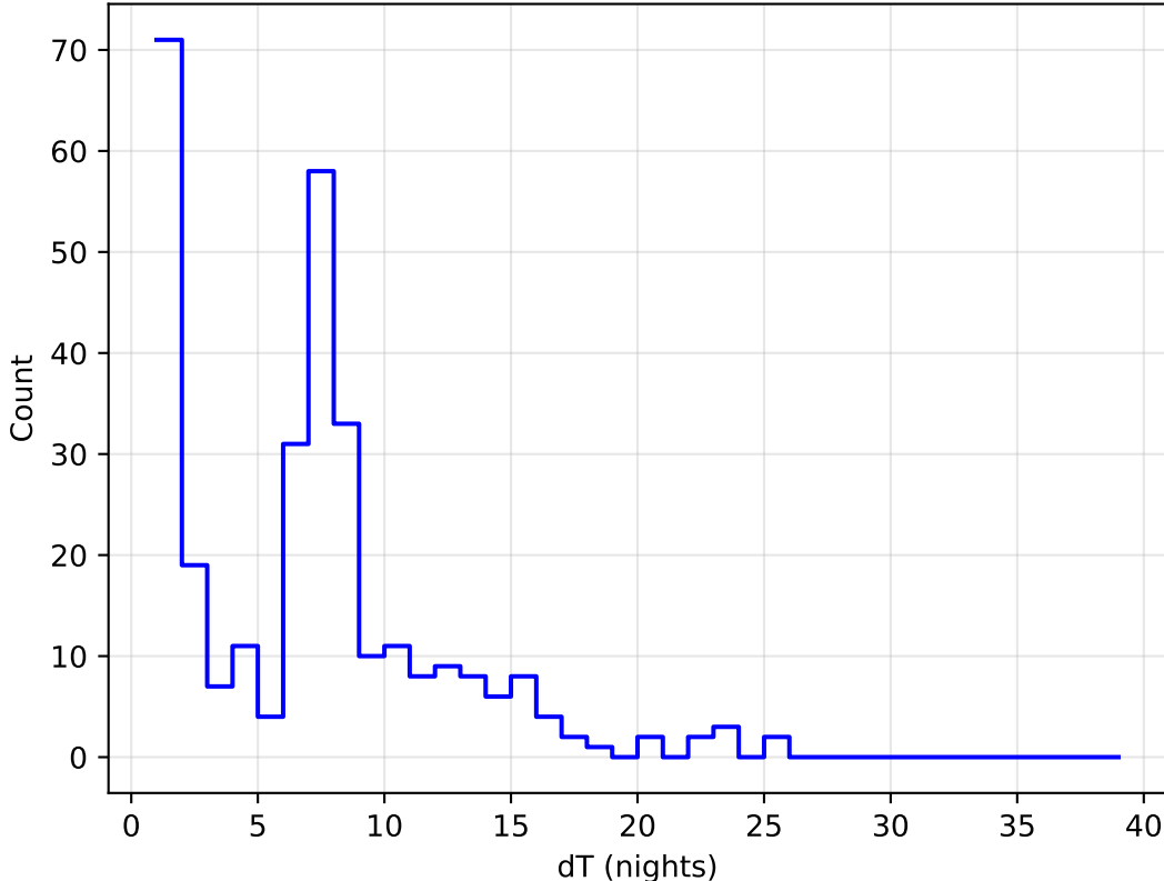
ddf_acor_sf10_lsf20_lsr10_v3.4_10yrs all bands: DD:XMM_LSS Delta Nights Histogram
