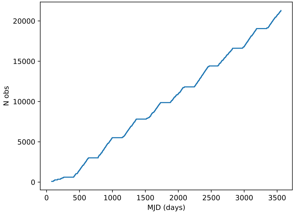
ddf_acor_sf10_lsf20_lsr10_v3.4_10yrs all bands: DD:ELAISS1 Cumulative NVisits
