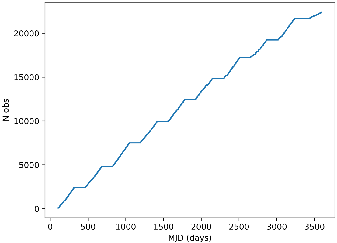
ddf_acor_sf10_lsf20_lsr10_v3.4_10yrs all bands: DD:EDFS Cumulative NVisits
