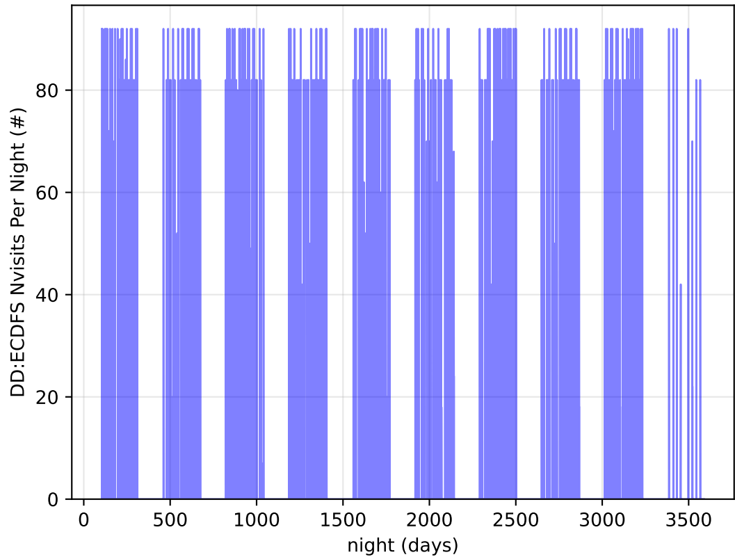
ddf_acor_sf10_ls10_lsr10_v3.4_10yrs all bands: DD:ECDFS Nvisits Per Night
