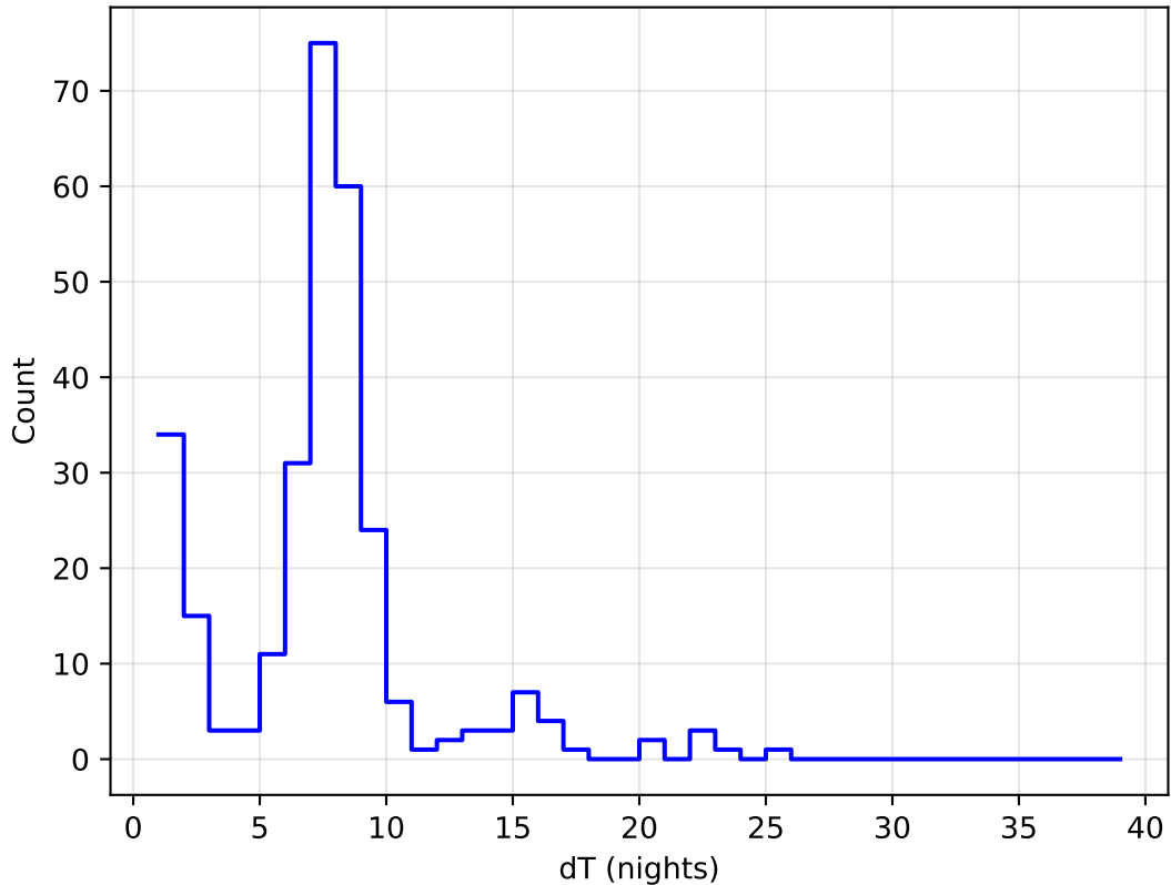
ddf_acor_sf10_lsf20_lsr10_v3.4_10yrs all bands: DD:ECDFS Delta Nights Histogram
