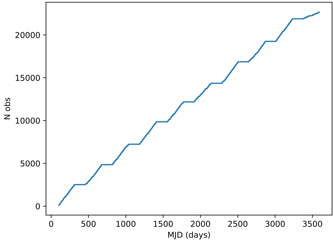
ddf_acor_sf10_lsf20_lsr10_v3.4_10yrs all bands: DD:ECDFS Cumulative NVisits
