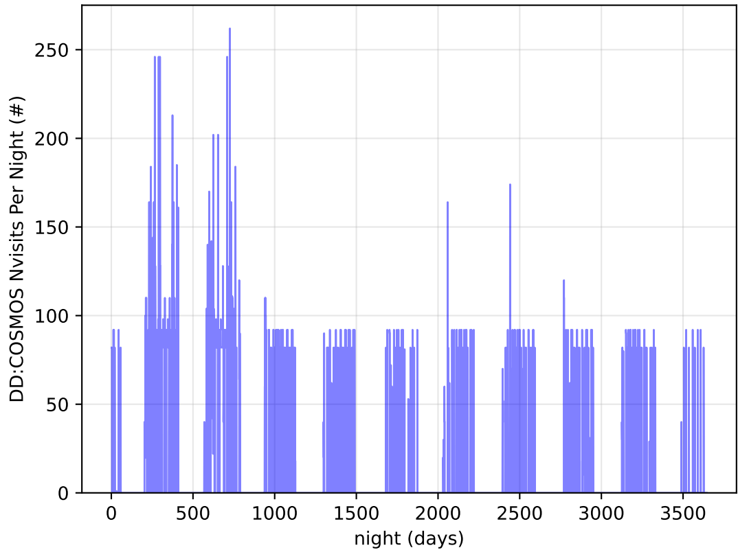
ddf_acor_sf10_lsf20_lsr10_v3.4_10yrs all bands: DD:COSMOS Nvisits Per Night
