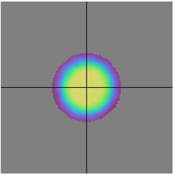
ddf_acor_sf10_lsf20_lsr10_v3.4_10yrs all bands: DD:COSMOS N Unique Nights
