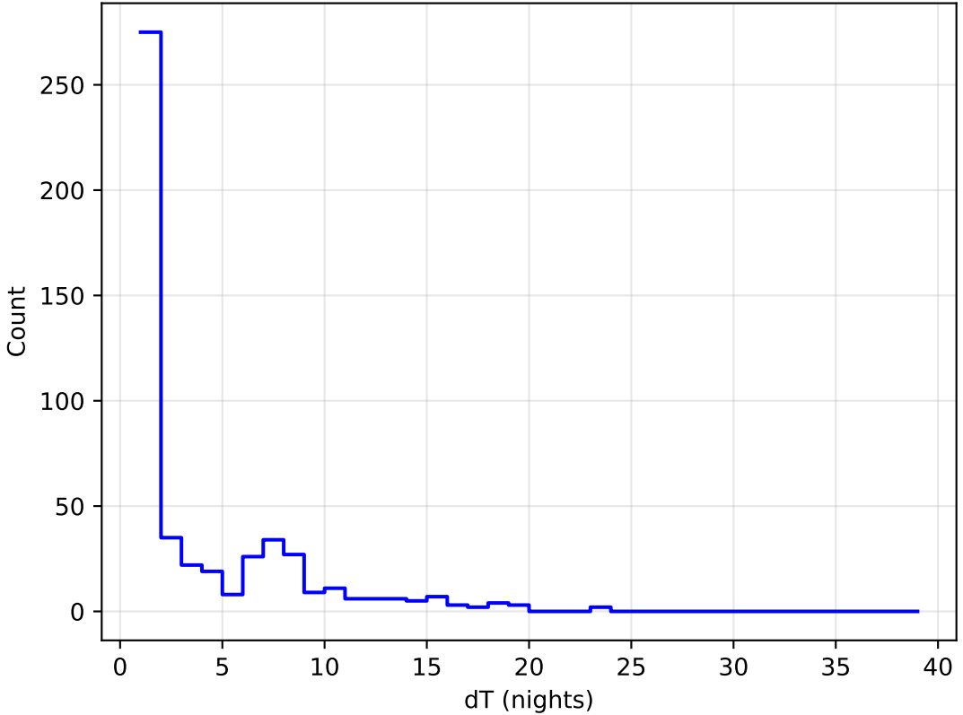
ddf_acor_sf10_lsf20_lsr10_v3.4_10yrs all bands: DD:COSMOS Delta Nights Histogram
