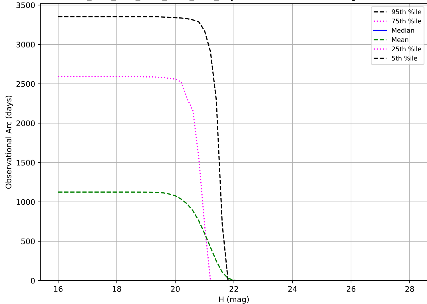
ddf_acor_sf10_lsf15_lsr50_v3.4_10yrs: Observational Arc Length Vatira
