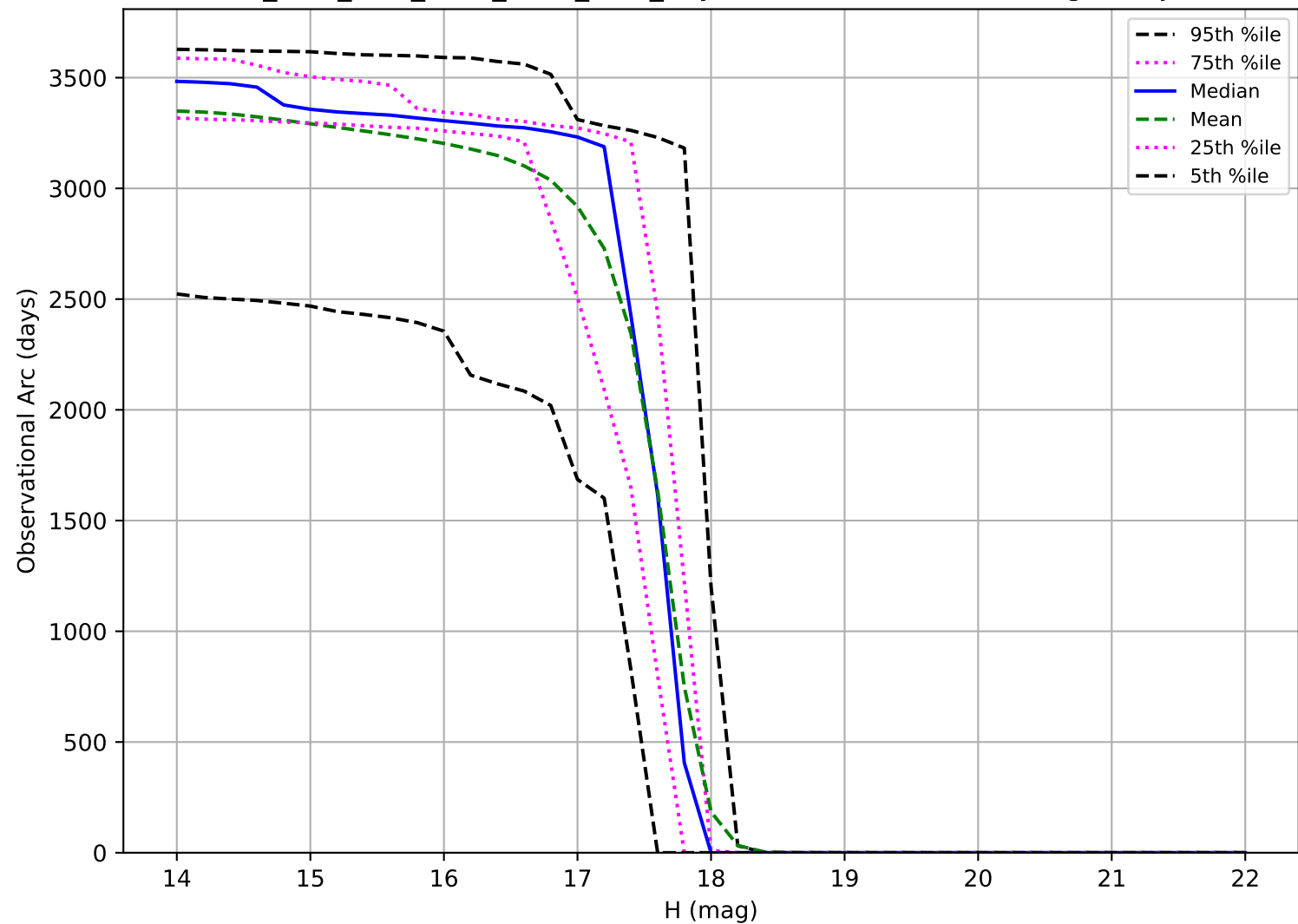
ddf_acor_sf10_lsf15_lsr50_v3.4_10yrs: Observational Arc Length Trojan
