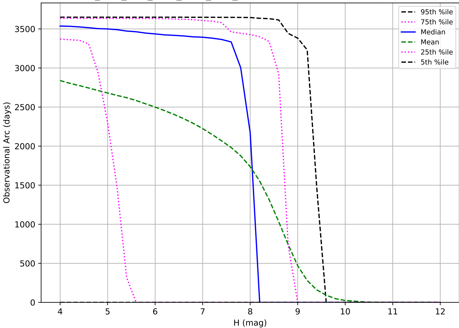
ddf_acor_sf10_lsf15_lsr50_v3.4_10yrs: Observational Arc Length TNO
