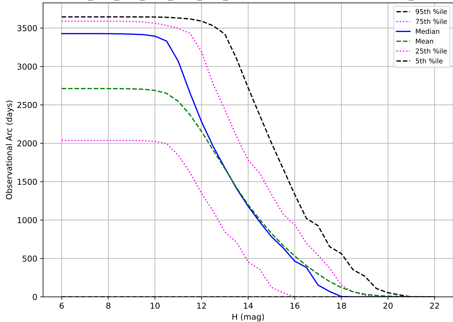
ddf_acor_sf10_lsf15_lsr50_v3.4_10yrs: Observational Arc Length OCC_r5
