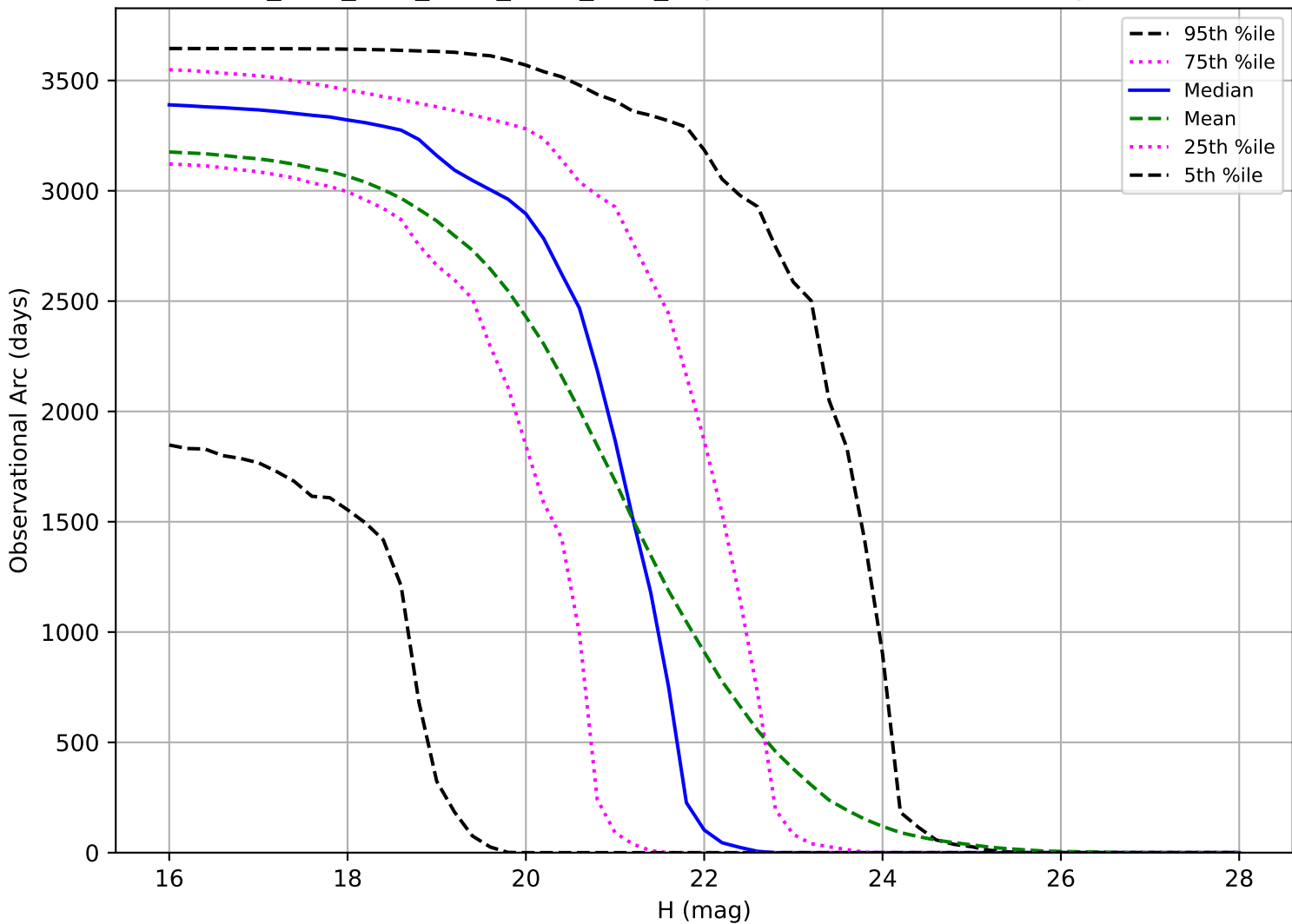
ddf_acor_sf10_lsf15_lsr50_v3.4_10yrs: Observational Arc Length NEO
