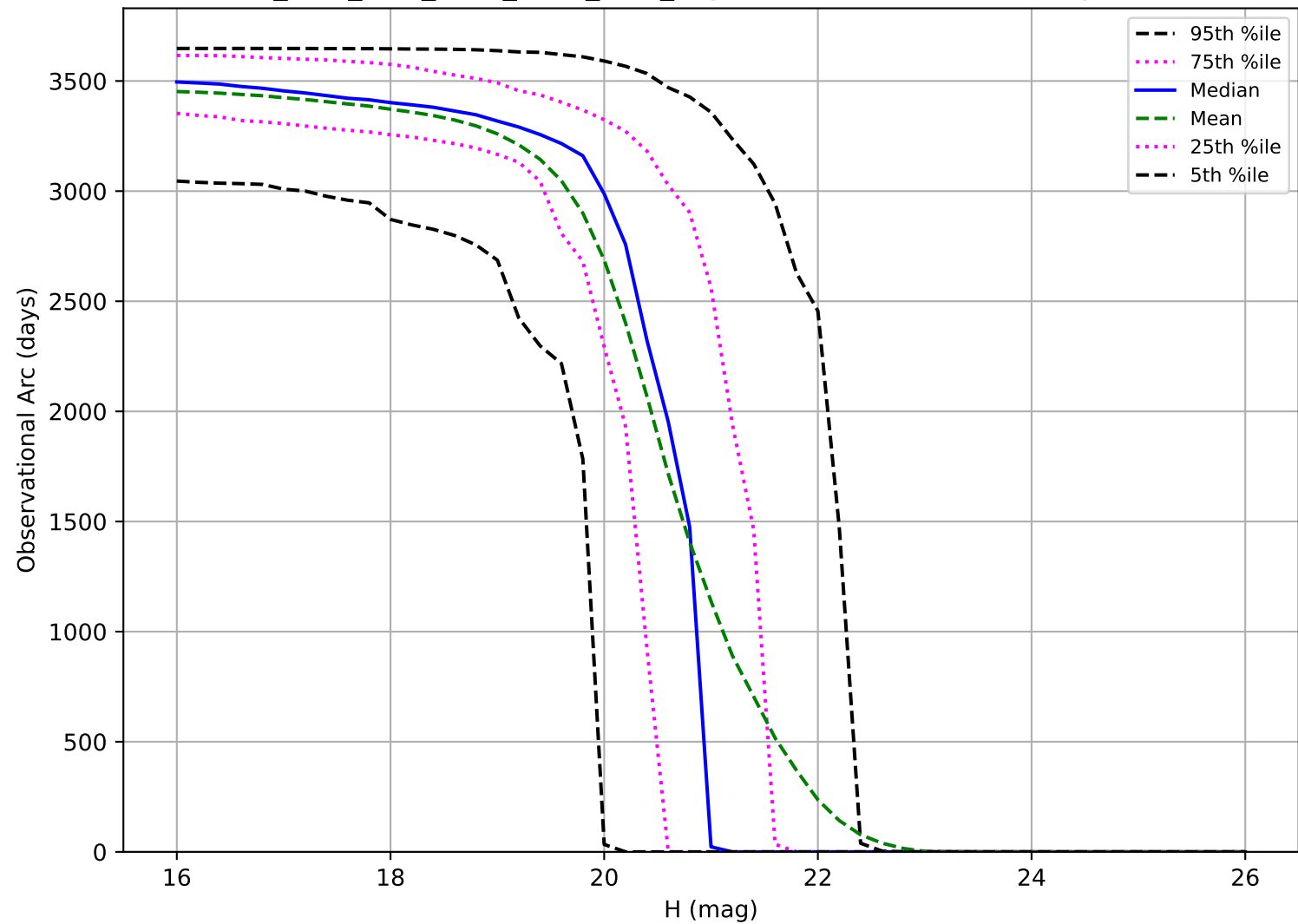
ddf_acor_sf10_lsf15_lsr50_v3.4_10yrs: Observational Arc Length MBA
