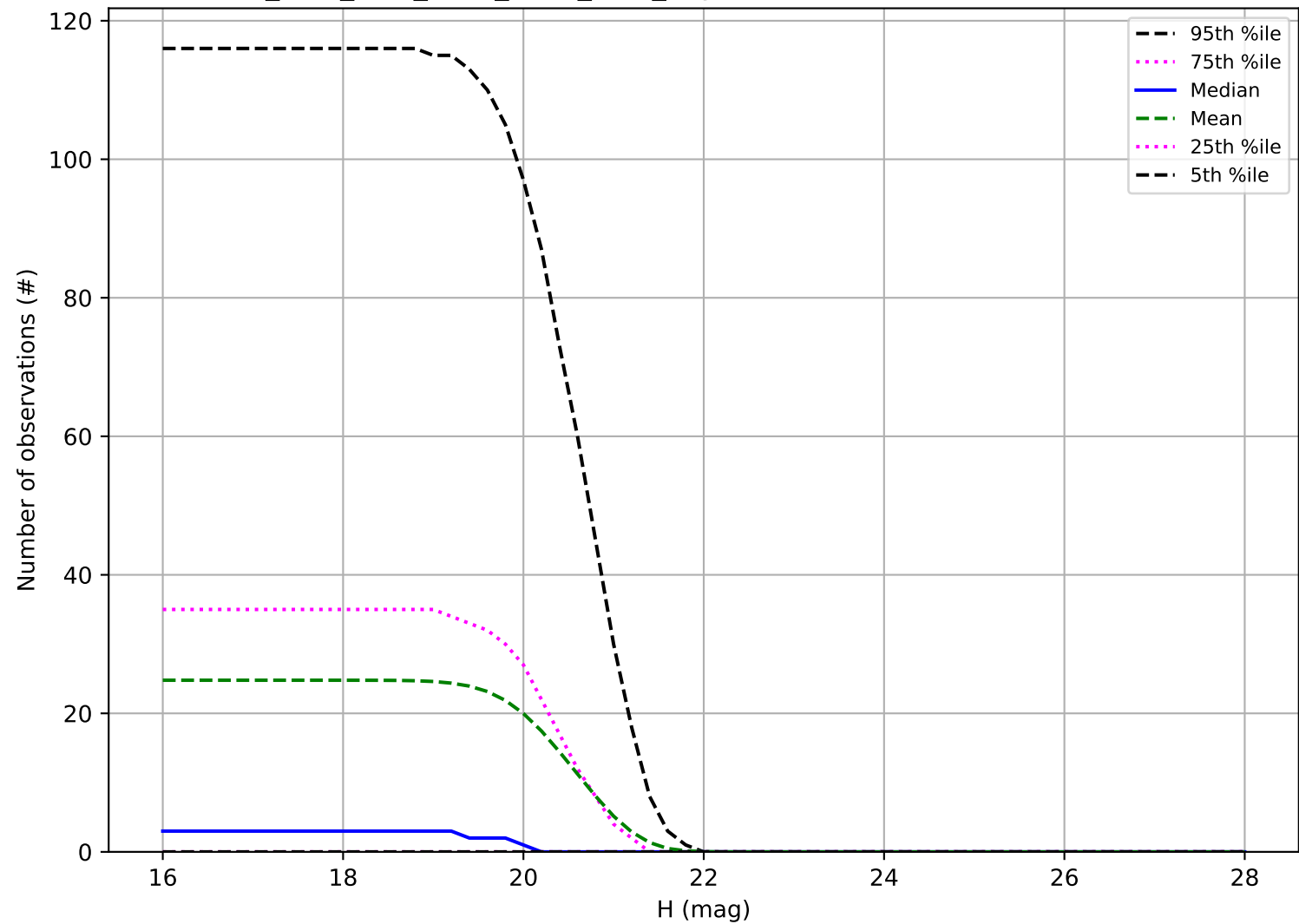
ddf_acor_sf10_lsf15_lsr50_v3.4_10yrs: Number of observations Vatira
