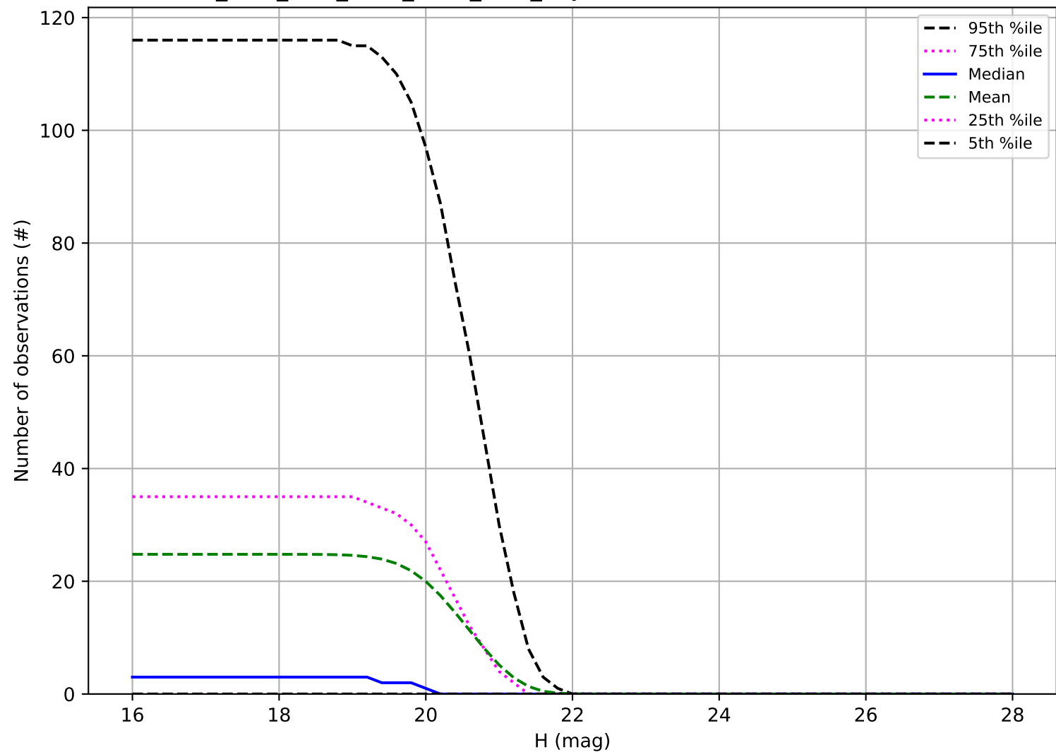
ddf_acor_sf10_lsf15_lsr50_v3.4_10yrs: Number of observations Vatira
